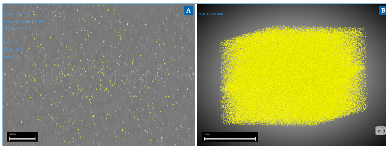
Figure 8. Particle distribution in NextDent Denture 3D Plus at 90°: (A) Representative 2D cross section, slice 709/810, 2.46 x 1.89 mm; (B) 3D view. Particles are highlighted in yellow.
