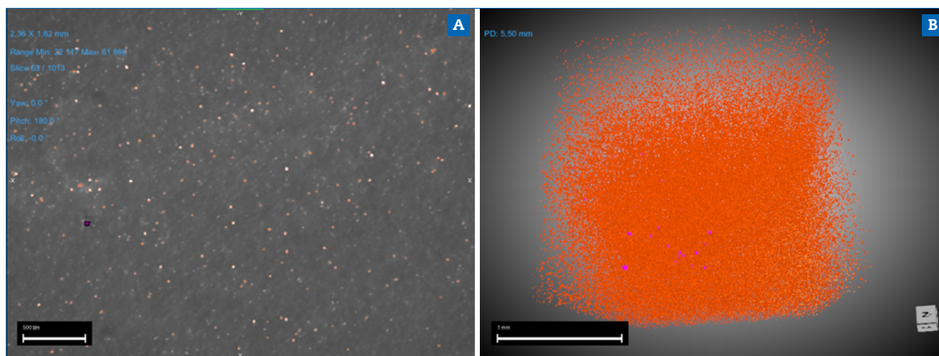
Figure 6. Particle distribution in NextDent Denture 3D Plus at 0°: (A) Representative 2D cross section, slice 63/1013, 2.36 x 1.82 mm; (B) 3D view. Particles are highlighted in orange.
