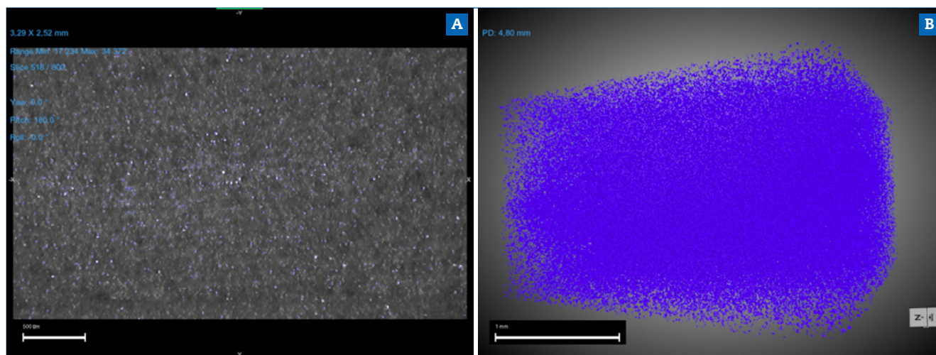
Figure 7. Particle distribution in NextDent Denture 3D Plus at 45°: (A) Representative 2D cross section, slice 518/800, 3.29 x 2.52 mm; (B) 3D view. Particles are highlighted in blue.
