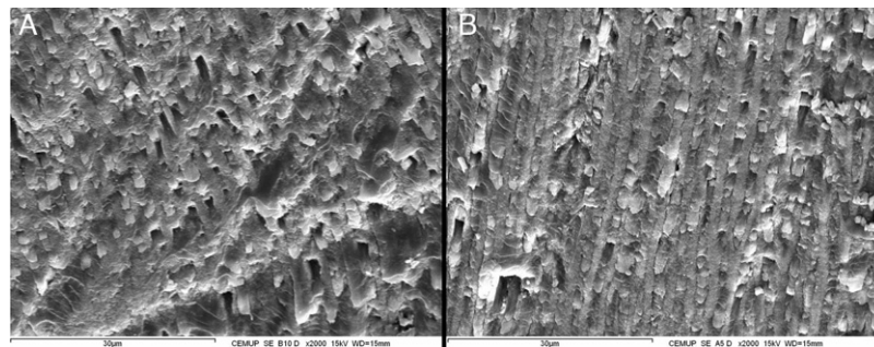
Fig. 2 – Enamel surface after being treated with the self-etching AdheSE® with (A) and without (B) Ozone. FESEM, 2000 \times , Gold. Enamel prisms can be identifiable in all the observed specimens.
