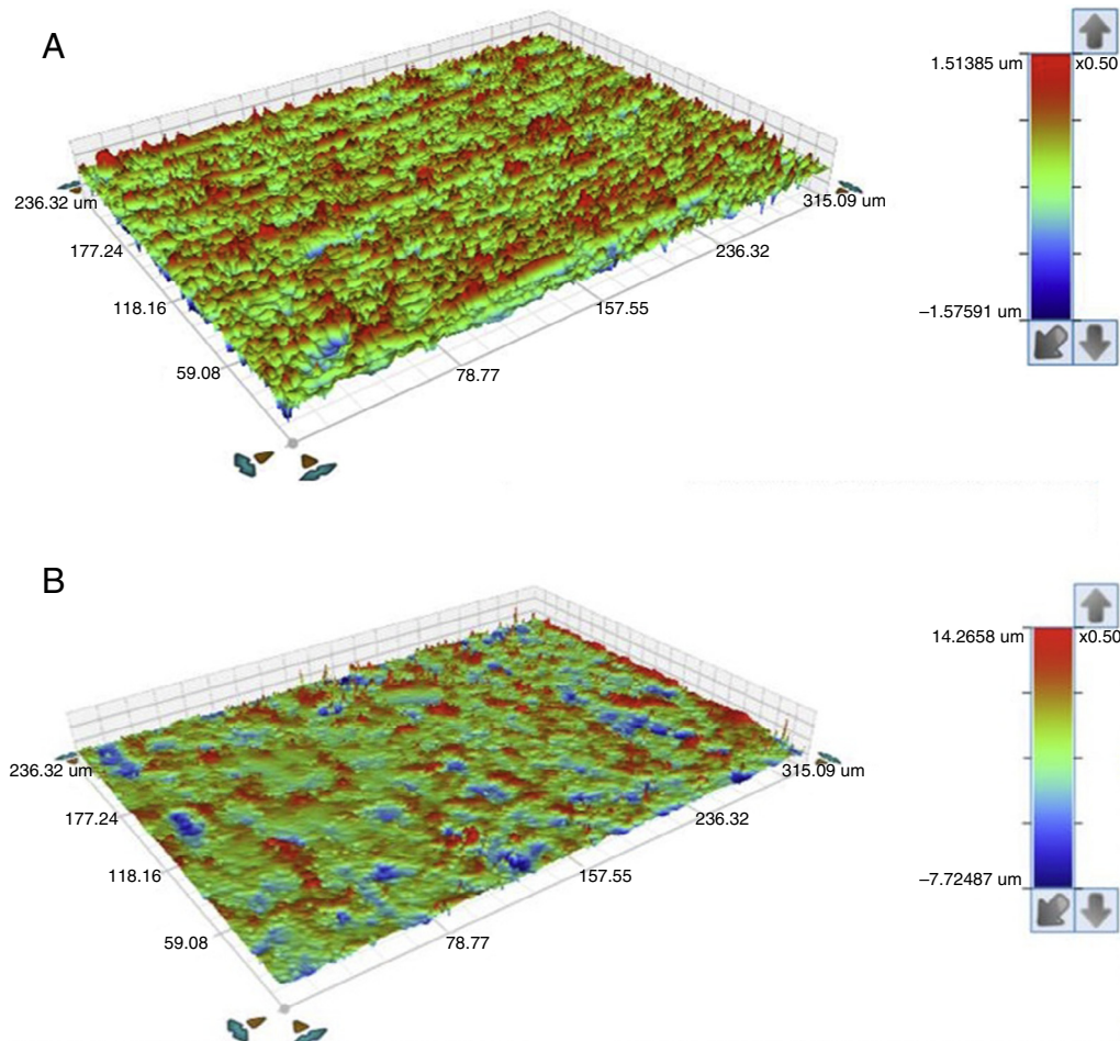
Figure 5 – 3D profilometry image of the seating platforms for external connection (A) and internal connection (B) abutments, at the initial state, in an area of measurement of 320 μm x 240 μm.
